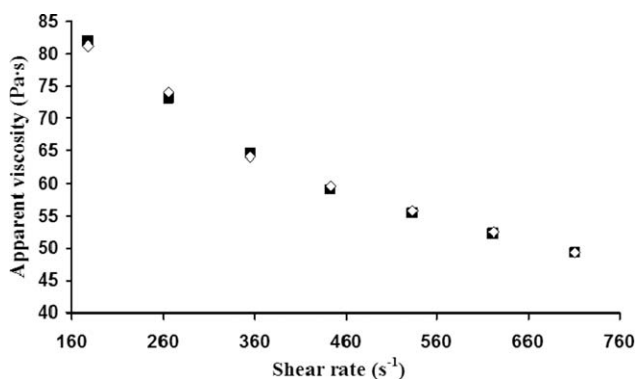
Figure 8. Apparent viscosity versus shear rate from duplicate measurements for the EVOH/FORSUD 5% samples (A2 in Table II).
