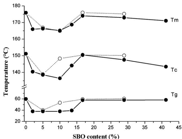
Figure 12. Temperature graph from DSC analysis versus SBO content for all composites (black circles for FORSUD and white circles for CVT230).
