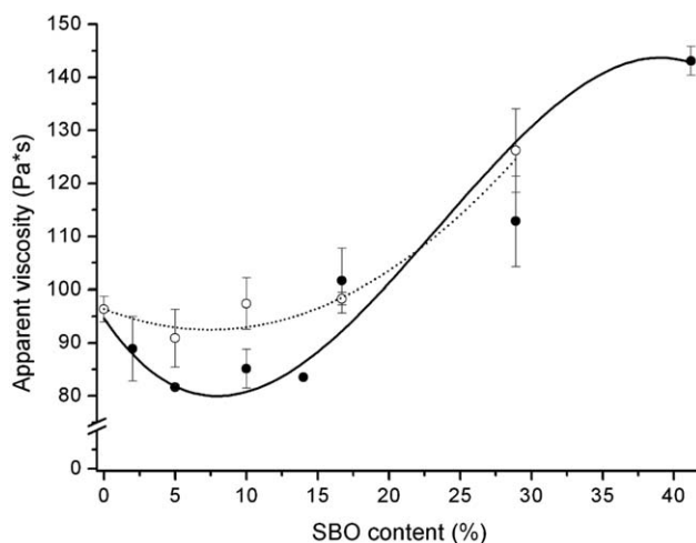
Figure 9. Apparent viscosity, measured at 50 rpm screw rotation speed (i.e., 177\text{ s}^{-1} shear rate), versus SBO content (black circles for FORSUD and white circles for CVT230) in the composites.
