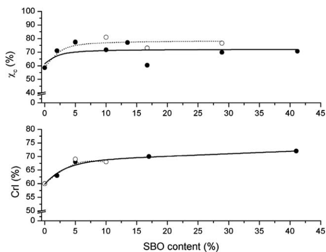
Figure 14. Crystallinity percentage versus SBO content weight % in EVOH-SBO extruded samples (black circles for FOR SUD and white circles for CVT230), calculated from melting enthalpies according to eq. (1) and from x-ray diffractograms according to eq. (2; CrI).
