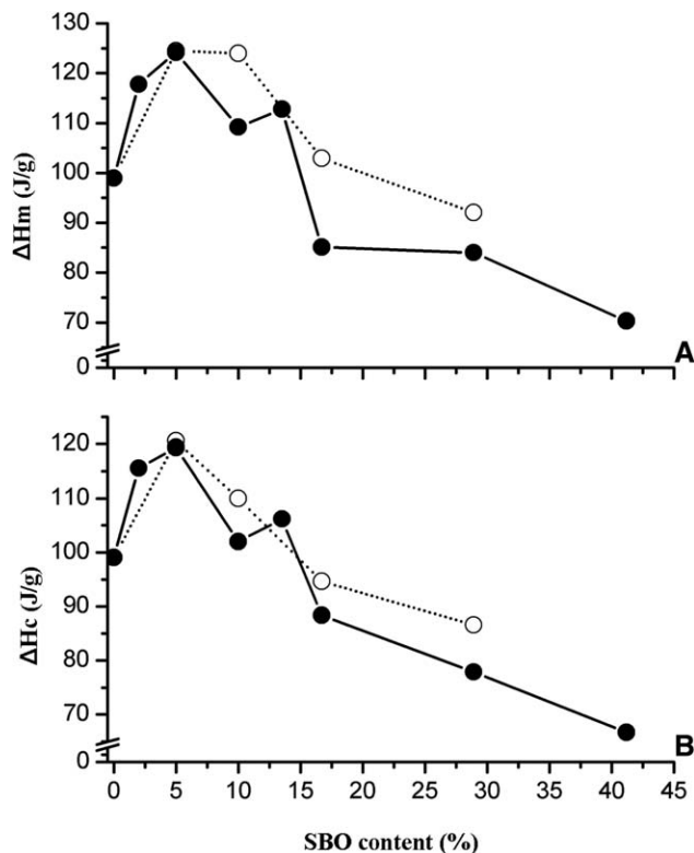
Figure 13. Melting (A) and cold crystallization (B) enthalpy graph from DSC analysis versus SBO content for all composites (black circles for FORSUD and white circles for CVT230).
