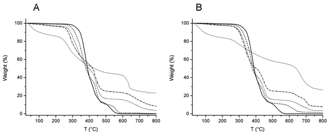
Figure 10. TGA scans reporting sample weight loss % upon increasing temperature for neat EVOH (solid black line), neat SBOs (gray line), and the EVOH blends with FORSUD (A) and CVT230 (B) at three different SBO concentrations, that is, 5% (dashed line), 17% (dotted line), and 29% (dot-dashed line).
